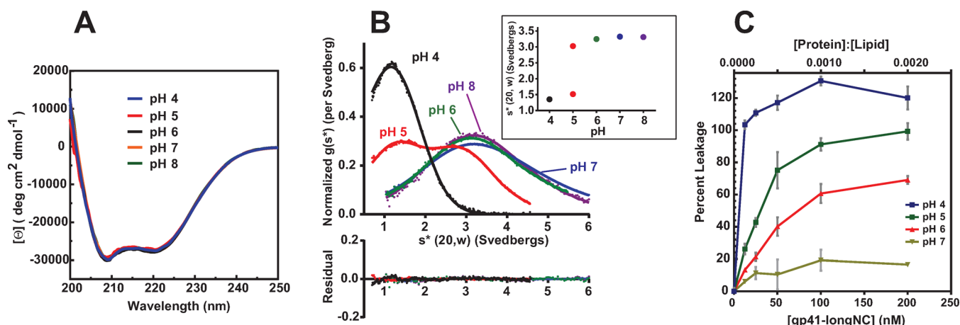
Figure 3. Properties of gp41-longNC. (A) CD, (B) AUC, and (C) liposome release assay under various pH conditions. For AUC, a monomeric species was observed at low pH (pH 4) and trimeric species were observed at higher pHs (pH 6, 7, and 8). At pH 5, both monomeric and trimeric species were observed, illustrated in the inset. All AUC experiments were performed at protein concentrations of 4–5 \mu M.
