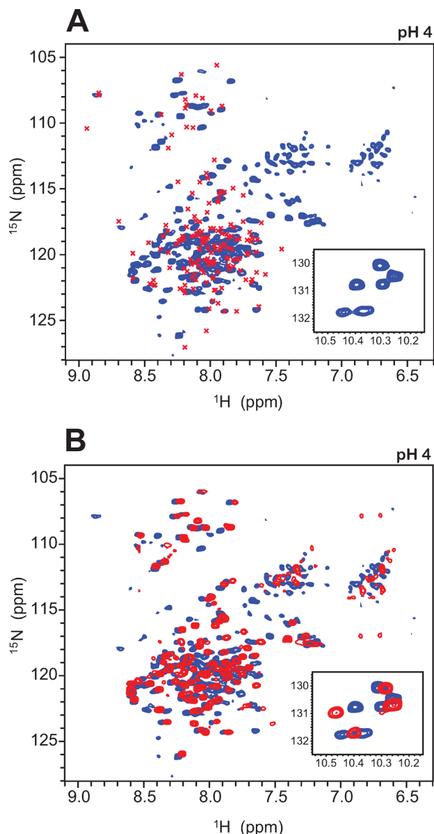
Figure 5. ^1\text{H}/^{15}\text{N} TROSY spectra of gp41-longNC and gp41-shortNC at pH 4. (A) TROSY spectrum of gp41-longNC (blue). The Trp side chain regions of the spectra are shown as insets. Previously reported cross-peak positions for similar gp41 constructs 12,19 are indicated with red crosses. (B) Overlay of the TROSY spectra for gp41-longNC (blue) and gp41-shortNC (red). Ninety percent of the gp41-shortNC cross-peaks fall near or on the corresponding resonance in gp41-longNC.
