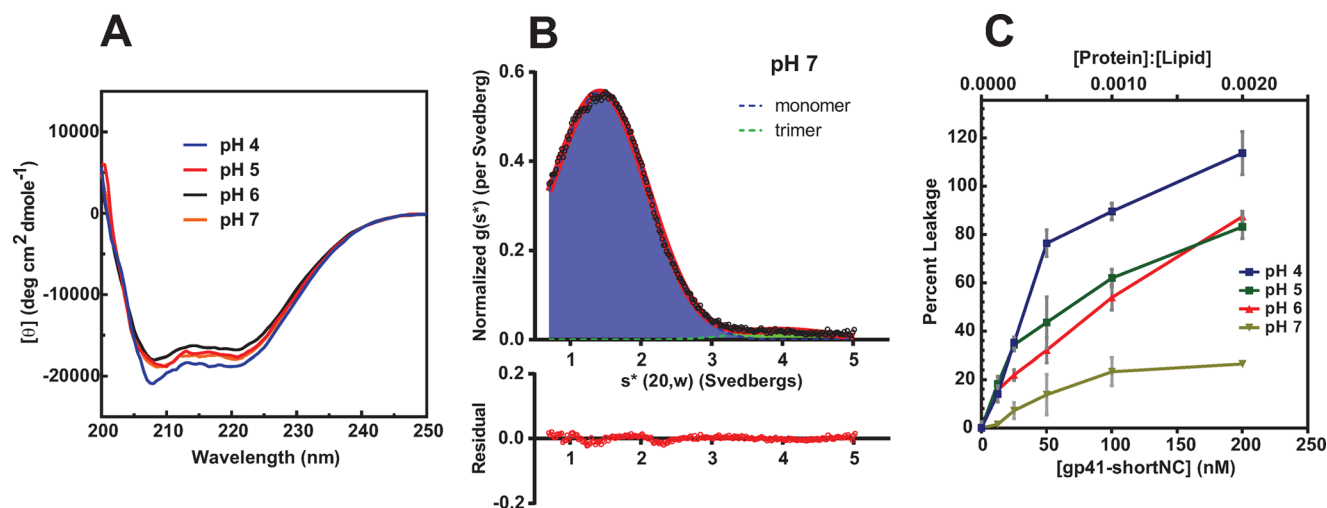
Figure 4. Properties of gp41-shortNC. (A) CD and (B) AUC at pH 7 and (C) liposome release assay under various pH conditions. For AUC data obtained at 21 \mu M gp41-shortNC (pH 7), the contributions from the monomer and trimer are colored blue and green, respectively.
