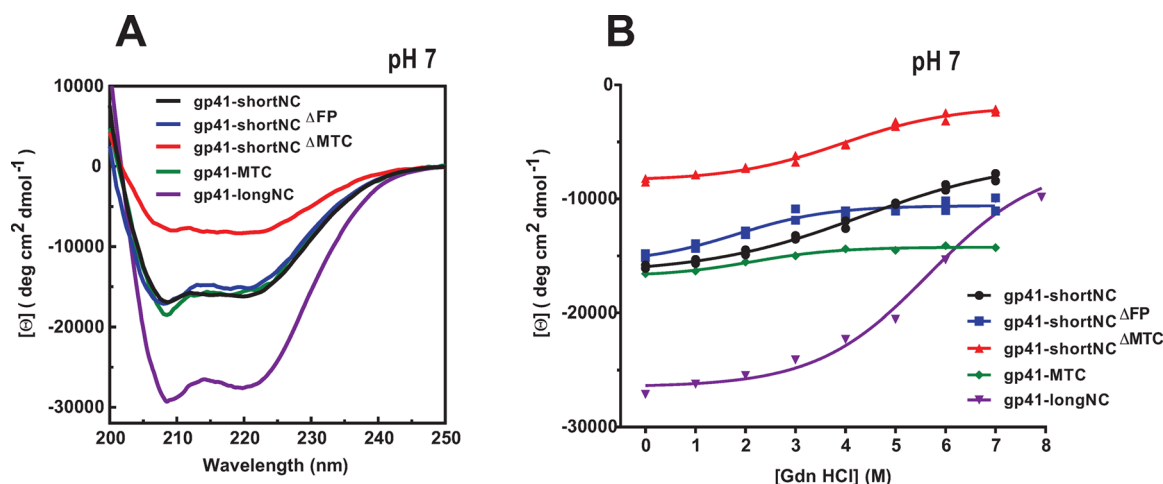
Figure 6. CD and chemical denaturation of gp41-shortNC, gp41-shortNC \Delta FP, gp41-shortNC \Delta MTC, gp41-MTC, and gp41-longNC at pH 7. (A) CD wavelength scans for gp41-shortNC \Delta FP, gp41-shortNC \Delta MTC, and gp41-MTC with data for gp41-shortNC and gp41-longNC included for comparison. (B) Chemical denaturation of all five constructs.
