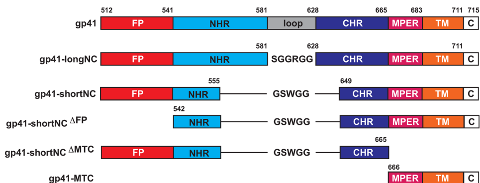
Figure 2. Schematic of HIV-1 gp41 and constructs studied. Abbreviations: FP, fusion peptide; NHR, N-heptad repeat region; CHR, C-heptad repeat region; MPER, membrane-proximal external region; TM, transmembrane region; C, C-terminal tail. HxB2 numbering is shown.
